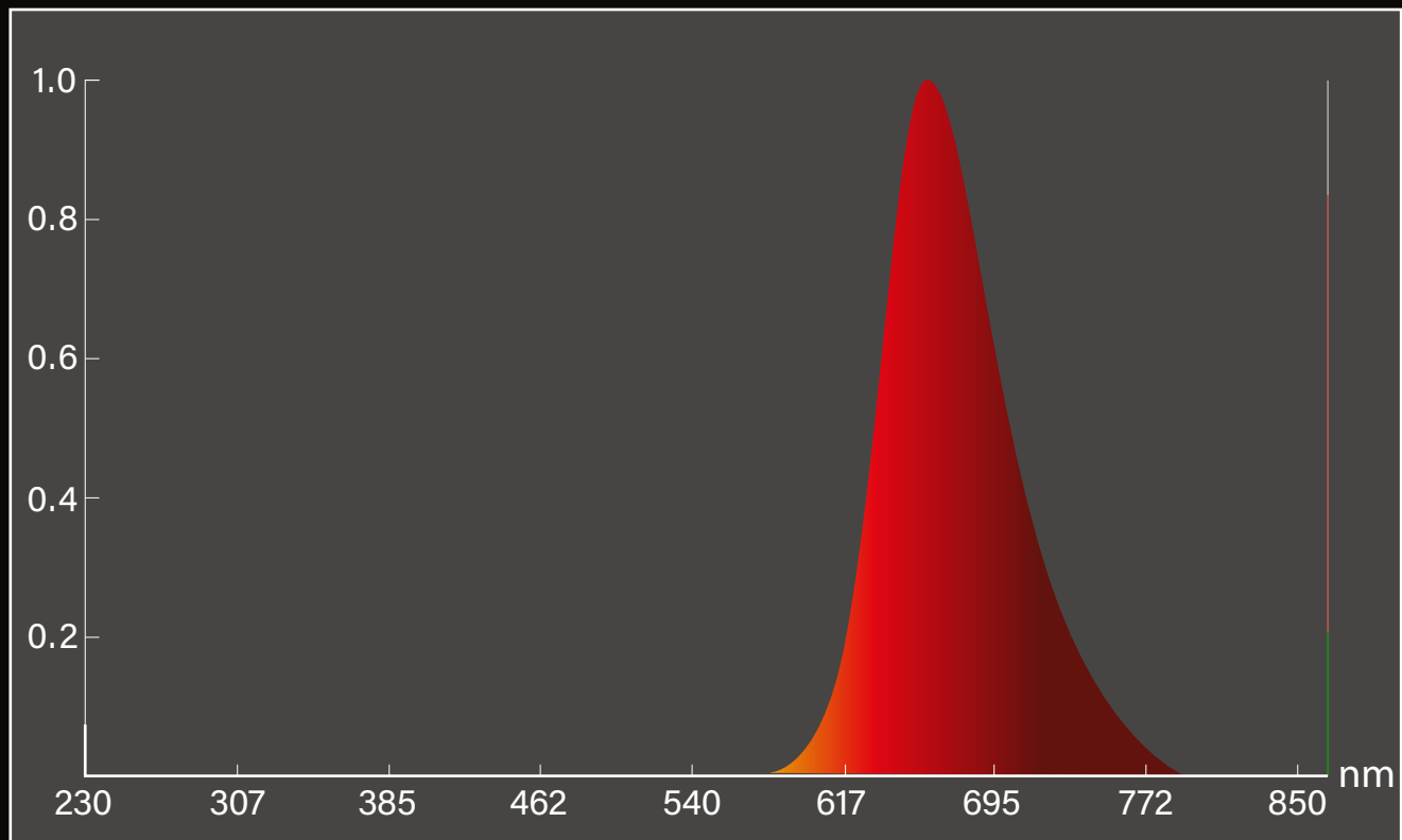
Spectrograma
